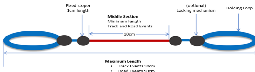
Figure 3 – Tether features
