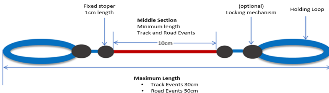
Figure 3 – Tether features
